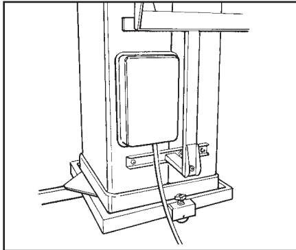
Relocated LVC box with main frame
